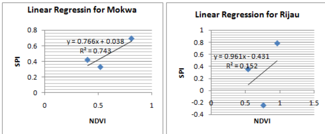
Figure 5: Linear Regressions for Mokwa and Rijau LGA.
