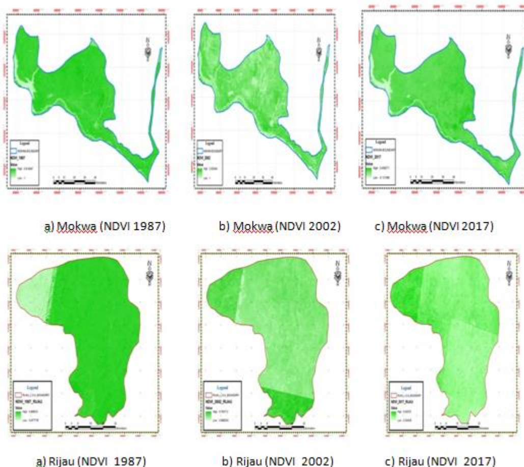
Figure 4: NDVI analysis for Mokwa and Rijau LGA. Source: Field Survey(2018)
