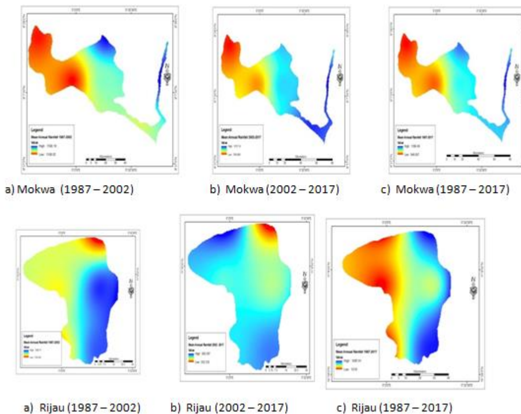
Figure 3: The spatial trends in mean rainfall from 1987 – 2017 in Mokwa and Rijau LGAs. Source: Field Survey (2018)
